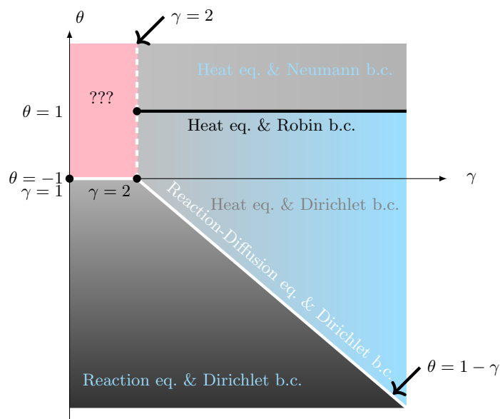
Fig. 7. Hydrodynamical behavior of the symmetric exclusion with long jumps.
