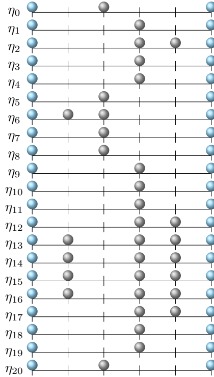
Fig. 1. Possible configurations starting from (0, 1, 0, 0)
