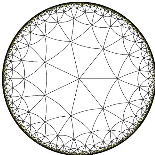
Figure 1: \mathbb{G}(7, 3, r)
